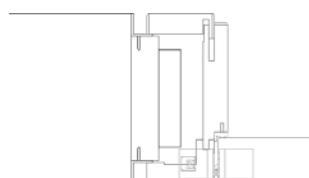
Blockzarge 60 mm
